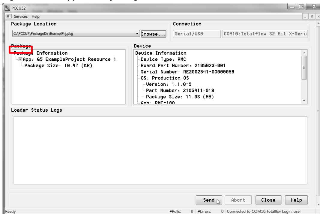
Figure 24: IEC application package selected in the G5 device loader
