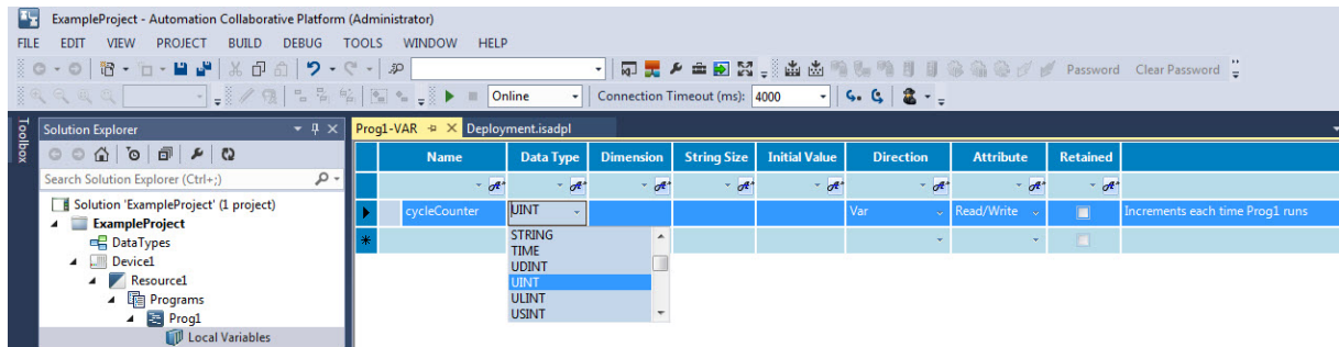
Figure 16: Add POU variables
