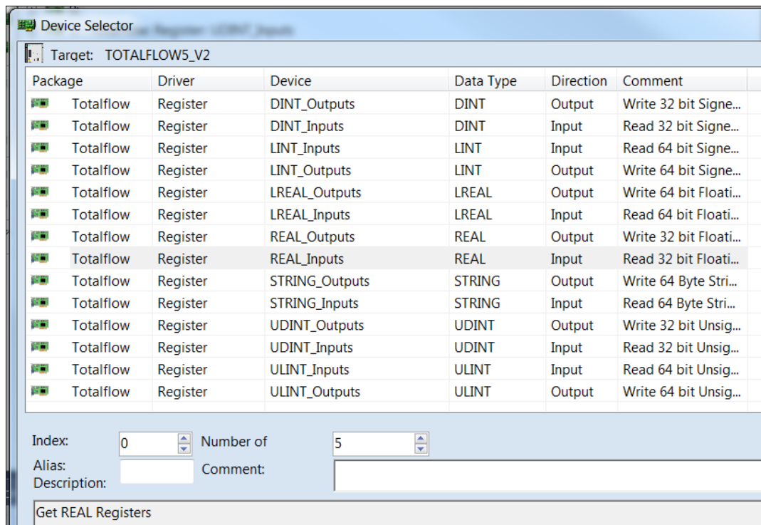
Figure 31: Device selector (available G5 I/O devices)
